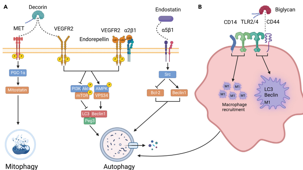
Figure 6. Schematic representation of the various proteoglycans and proteoglycan fragments evoking autophagy
