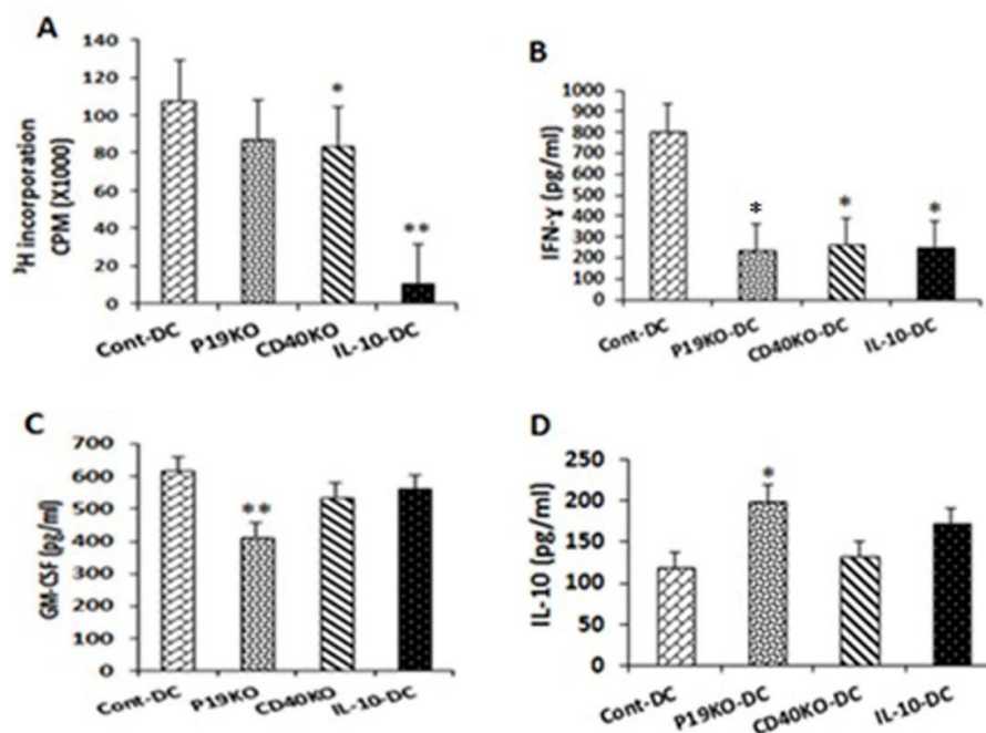
Figure 4. CD40KO and IL-23p19KO BMDCs have reduced capacity to stimulate IFN- \gamma production by CD4 ^{+} T cells. A) CD40KO, IL-23p19KO and IL-10-treated DCs were co-cultured with 2D2 CD4 ^{+} T cells at a T cell:DC ratio of 4:1 for 3 days. ^3 H-thymidine was added to the cultures for the last 24 h. Data are presented as the mean values of triplicate cultures \pm SEM. B), C), and D) IFN- \gamma , GM-CSF, and IL-10 were measured in the supernatants of separate CD4 ^{+} T cell-DC co-cultures by ELISA. * P <0.05 and ** P <0.01 represent statistically significant difference between test co-cultures with test DCs and Cont-DCs. The results shown are representative of two independent experiments
