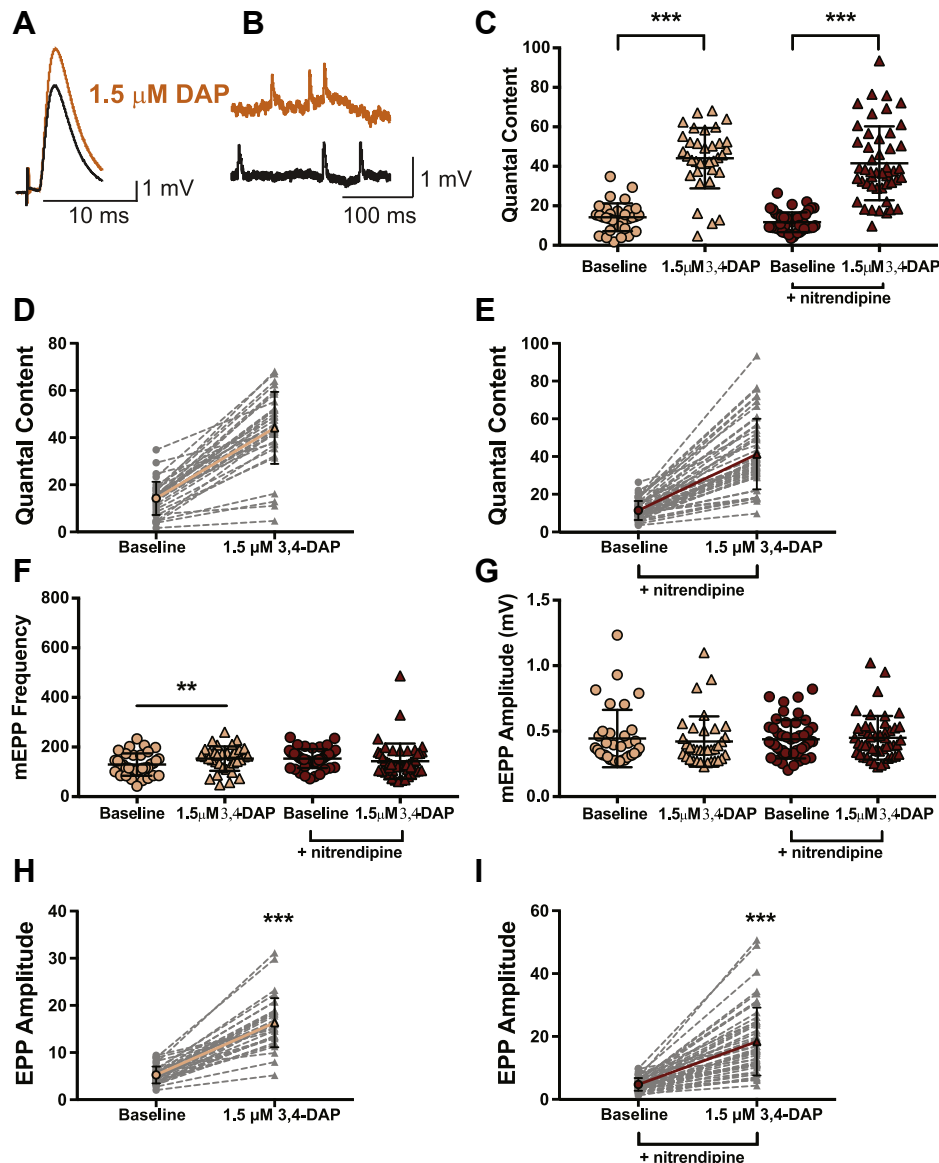
Figure 5. 1.5- \mu M 3,4-DAP dose dependently increases neuromuscular transmission independent of Cav1 channels in mouse neuromuscular junctions. A and B, sample traces of electrophysiological recordings of EPPs (A) and mEPPs (B) before and after 1.5- \mu M 3,4-DAP application. C, quantified quantal content before (circles) or after (triangles) 1.5- \mu M 3,4-DAP application to vehicle (peach) or nitrendipine (red) treated mouse NMJs. Two-way mixed ANOVA was used (there was a significant main effect of 1.5- \mu M 3,4-DAP (F (1, 81) = 347.5, *** p < 0.0001); no significant main effect of nitrendipine (F (1, 81) = 1.136, p = 0.2897) or interaction between 3,4-DAP and nitrendipine (F (1, 81) = 0.0002, p = 0.9887); vehicle, n = 35; nitrendipine n = 48). D and E, plots of individual paired values (gray dotted lines) with a superimposed average (solid peach line, vehicle; solid red line, nitrendipine). F, there was a significant interaction between the effects of 1.5- \mu M 3,4-DAP and nitrendipine on mEPP frequency (two-way mixed ANOVA; no main effect of nitrendipine; F (1, 81) = 0.4209, p = 0.5183) or 3,4-DAP; F (1, 81) = 1.634, p = 0.2048), but a significant interaction between 3,4-DAP and nitrendipine (F (1, 81) = 10.02, p = 0.0022). Post hoc simple main effect analysis showed a significantly increased mEPP frequency in the vehicle (peach, ** p = 0.0090) but not the nitrendipine (red, p = 0.3004) condition. G, the 1.5- \mu M dose of 3,4-DAP did not significantly alter mEPP amplitude in vehicle (peach) or nitrendipine (red) conditions; two-way mixed ANOVA (no significant main effect of nitrendipine; F (1, 81) = 0.08568, p = 0.7705, or 3,4-DAP; F (1, 81) = 0.2994, p = 0.5857, or significant interaction between 3,4-DAP and nitrendipine; F (1, 81) = 2.45, p = 0.1214). H and I, the 1.5- \mu M dose of 3,4-DAP increased EPP amplitude, shown as individual pairs (gray dotted lines) with a superimposed average (solid peach line, vehicle, H; solid red line, nitrendipine, I); Wilcoxon signed-rank test, *** p < 0.0001. 3,4-DAP, 3,4-diaminopyridine; Cav, voltage-gated calcium; EPP, endplate potential; mEPP, miniature EPPs; NMJ, neuromuscular junction.
