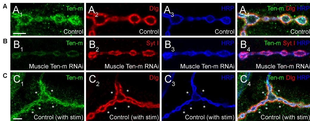
FIGURE 4 | Presynaptic Ten-m localizes to newly formed synaptopods. Single confocal sections of NMJs stained with antibodies to Ten-m (green), Dlg (red), and HRP (blue, in A,C ) or Ten-m (green), Syt I (red), and HRP (blue, in B ). Control NMJs show predominantly postsynaptic Ten-m localization ( A ) but a presynaptic component associated with the HRP-positive membrane and synaptic vesicle (via Syt I) population is visible upon genetic removal of the postsynaptic pool of Ten-m ( B ). Following spaced stimulation, Ten-m (green) is visible within newly formed synaptopods (marked by asterisks) that have not yet been apposed by postsynaptic Dlg (red) staining. Scale = 5 \mu m.
