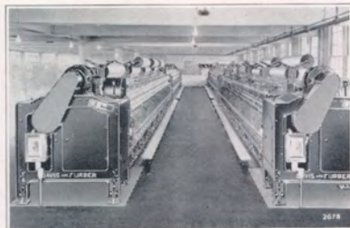
Ring Spinning Frame for All Materials Spun on the Woolen System
