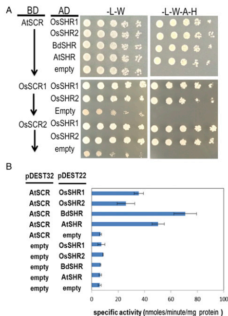
Fig. 4. The SHR homologs interact with SCR. (A) Fivefold serial dilutions of diploid yeast expressing AtSCR, OsSCR1, or OsSCR2 as bait with the SHR prey proteins (as labeled) grown on selective medium. Medium lacking adenine and histidine was used to select for interaction between the bait and prey proteins. AD, activation domain vector (prey); BD, binding domain vector (bait). BiFC results are shown in Fig. S5A. (B) Quantitative beta-galactosidase assays showing the specific activity of the beta-galactosidase enzyme induced by the interaction of the bait and prey proteins. The interacting proteins are as labeled. Assays were done in diploid yeast and normalized to total protein.
