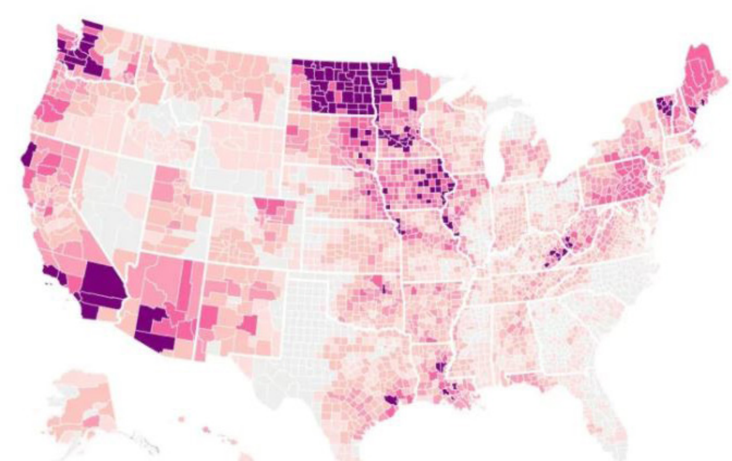
Floods
