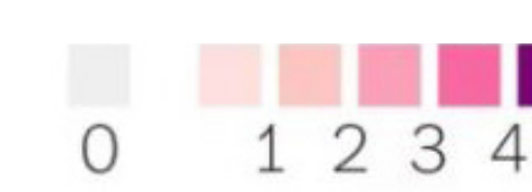
Tornadoes
