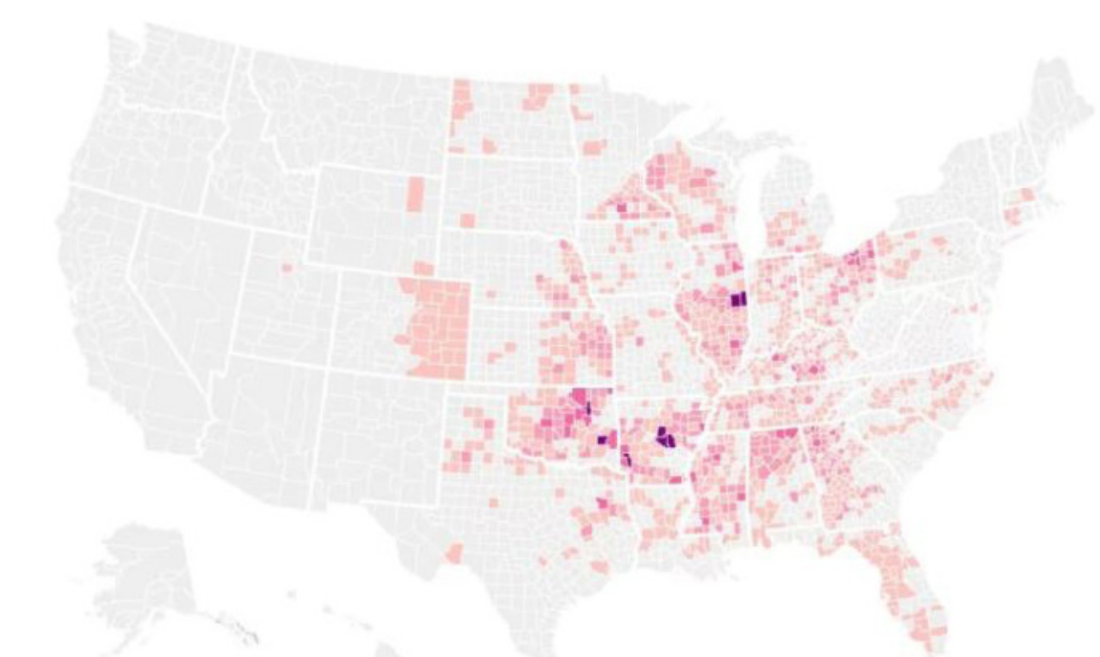
Tornadoes
